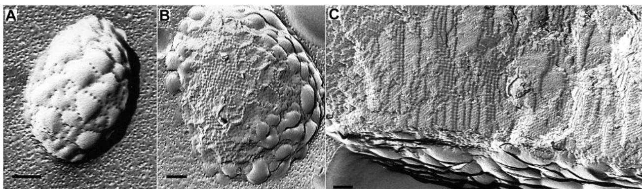
FIGURE 6 Equimolar mixtures of DODAC/CHEMS adopt nonbilayer structures after hydration at neutral pH values. Freeze-fracture electron micrographs of equimolar mixtures of DODAC/CHEMS hydrated in 50 mM HEPES, 150 mM NaCl (pH 8.1) reveal (A and B) lipidic particle structures and (C) regular arrays of lipidic particles. Freeze-fracture replicas were prepared and observed as described in Methods and Materials. Scale bars: 200 nm.
